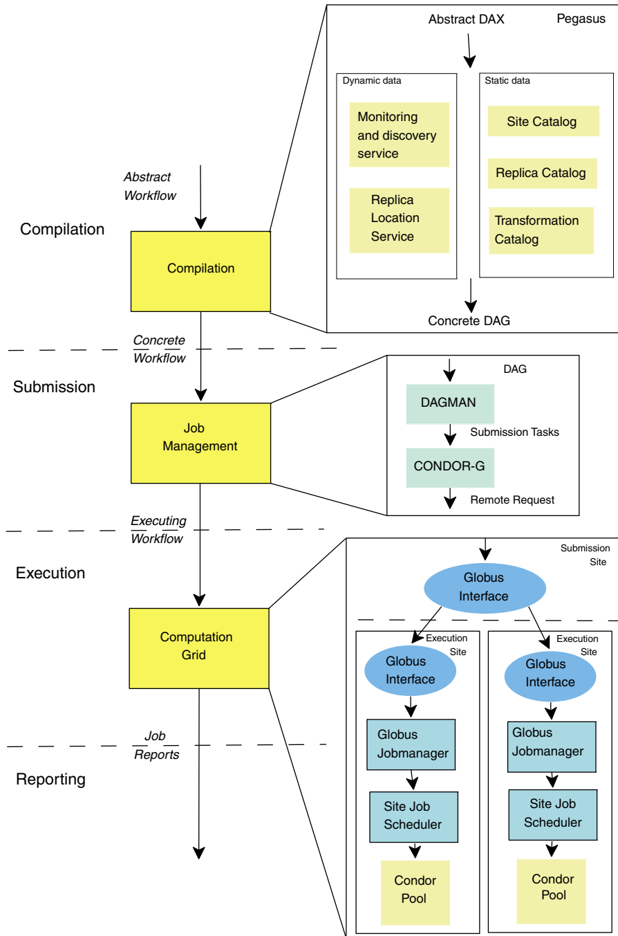
Figure 1. Workflow execution using Pegasus.
